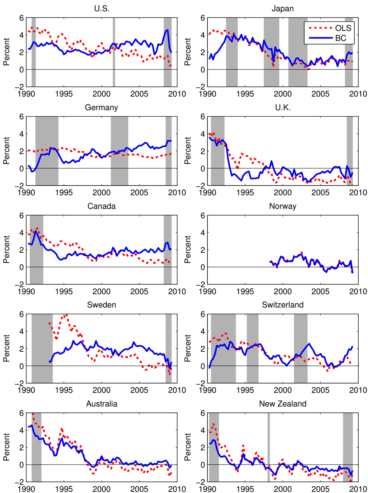
Figure 2: Term premia
